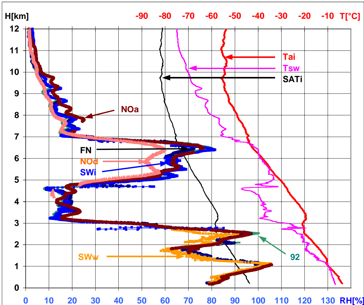
Fig.1: Comparison of nighttime FN-SW-92-NO relative humidity profiles in the Arctic troposphere in the height range 0.18 - 12 km, Sodankylä, 15.02.04, 17:25 ascent. Details are presented in Fig.2 (0 - 2 km), Fig.3 (2 - 4 km), Fig.4 (4 - 6 km), Fig.5 (6 - 8 km),
